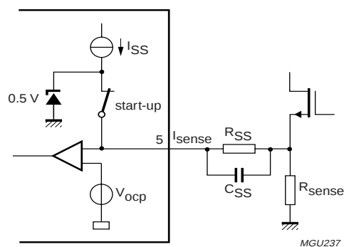
Fig.10 Soft start.
